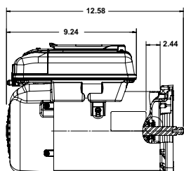
ECM16SQU EPA16SQ
